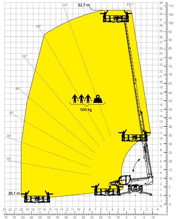
Load chart with ROTATING EXTENDABLE PLATFORM, 500 kg ATT - 01 - 005
